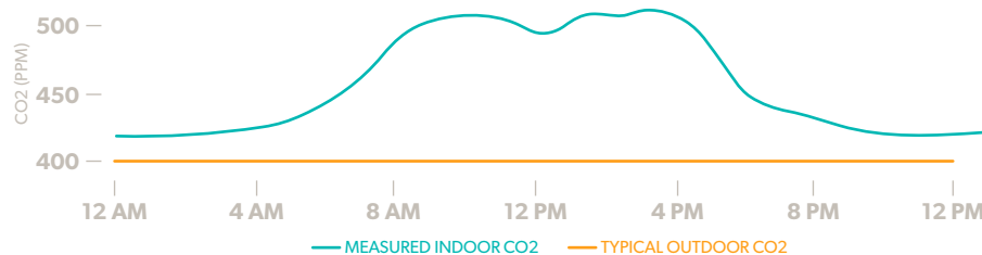
Average Weekday Indoor CO 2 Level
