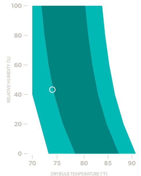
Temperature-humidity Chart
